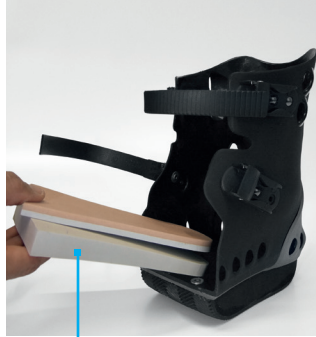
Wedge-shaped sole system for optimal rear weight-bearing
